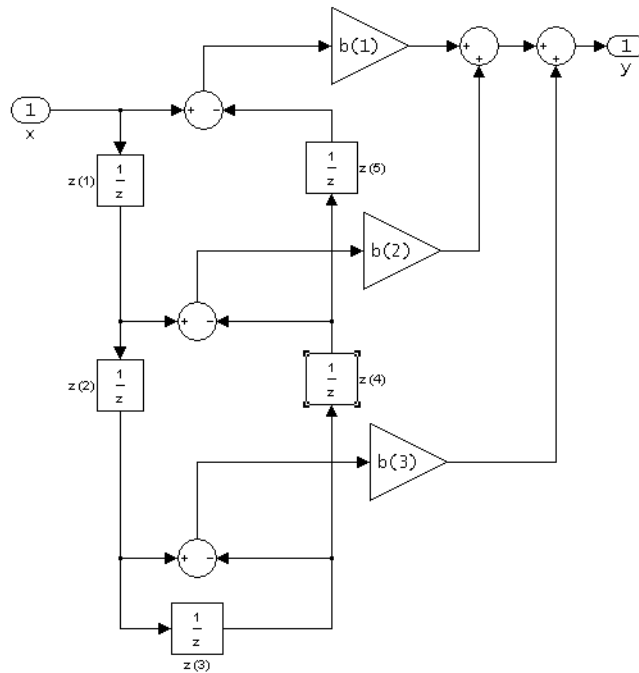
dfasymfir (Antisymmetric FIR) Even number of coefficients, length(b) = 6
