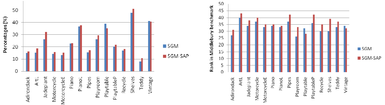
Figure 3. Errors for all stereo-pairs (left) and ranking in Middlebury benchmark (right) for SGM and our method (SGM-SAP).
