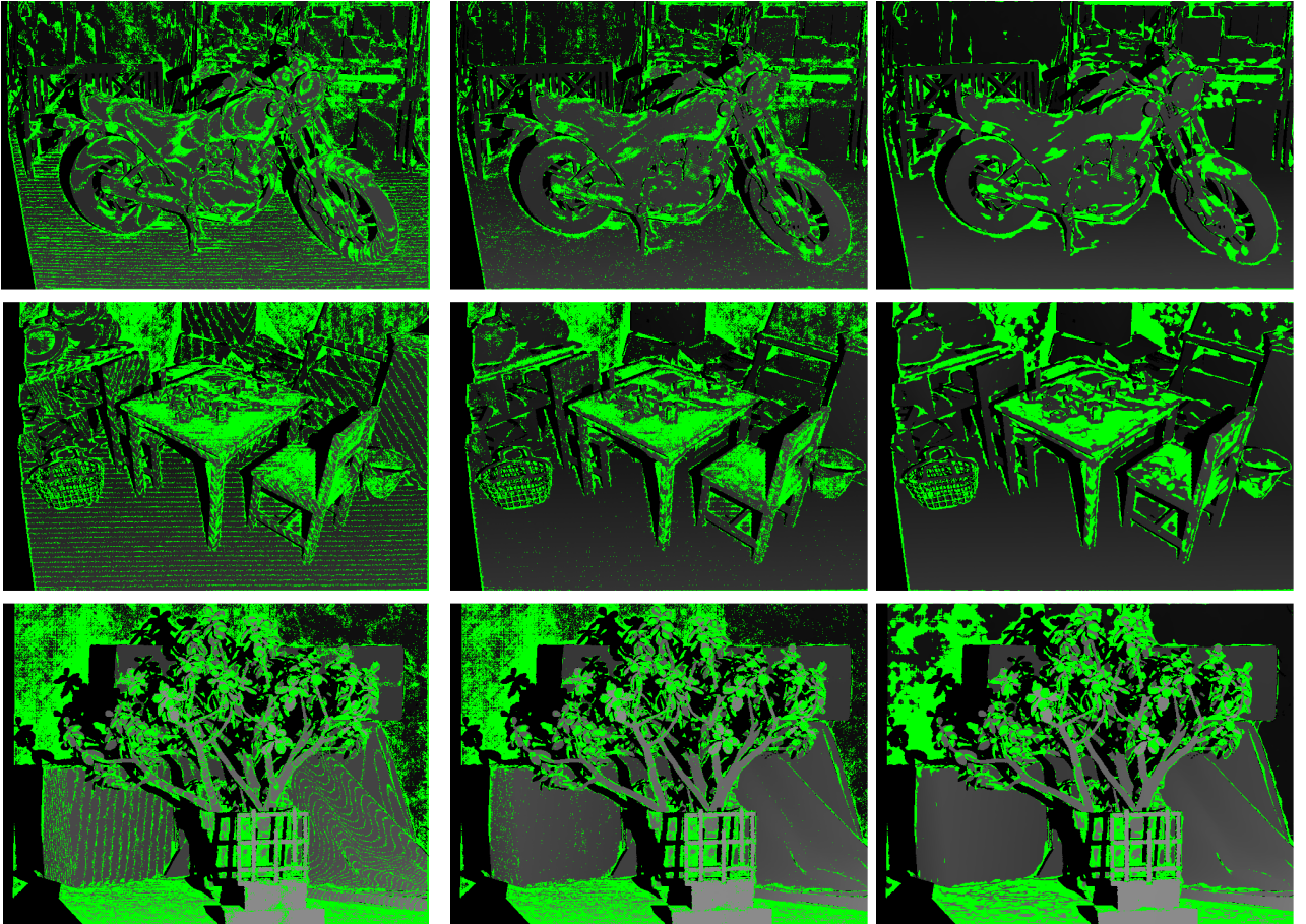
Figure 1. Estimated disparity maps using SGM-SAP. Left : disparity maps without any refinement; centre : sub-pixel interpolation; right : median filtering. Differences above 0.5 pixel from the ground truth are highlighted in green. Top to bottom : Motorcycle , PlayableP and Jadeplant stereo-pairs.
