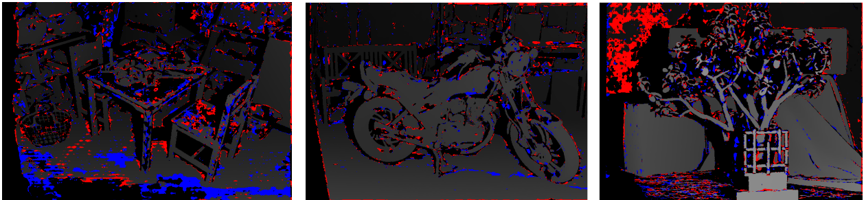
Figure 4. Disparity maps of the suggested method (from left to right: Playtable , Motorcycle and Jadeplant stereo pairs). Pixels in blue indicate errors of SGM algorithm which do not exist in our method; pixels in red depict errors of our method not present in SGM.
