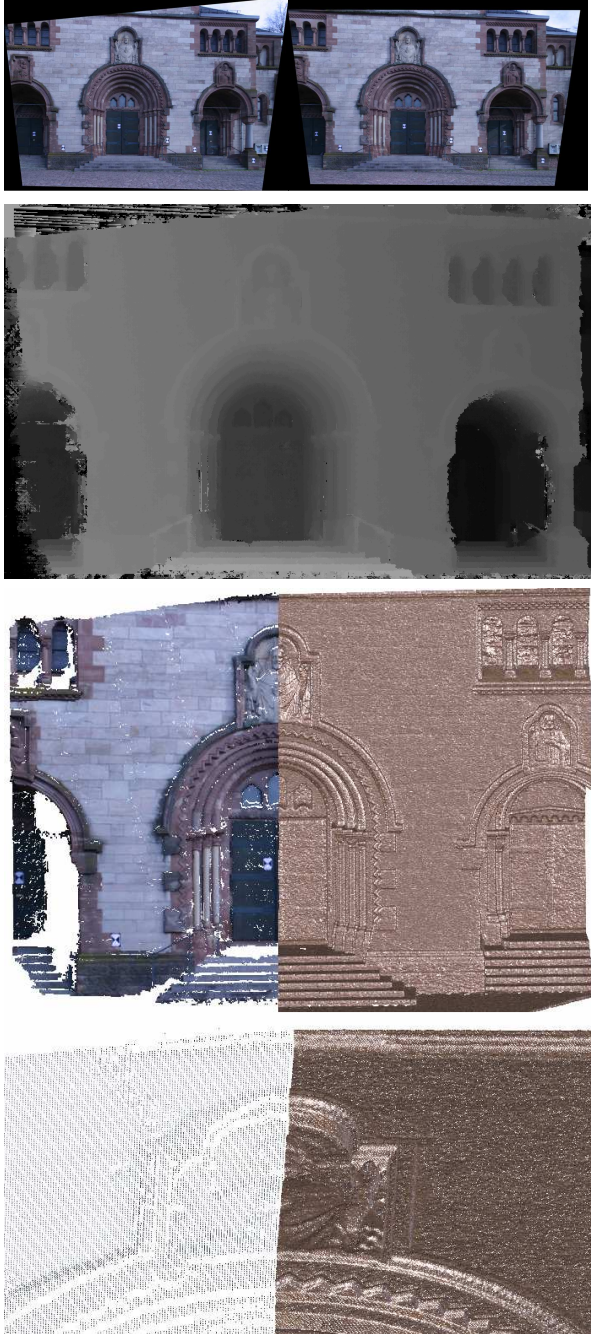
Figure 6. Results of SGM-SAP on the Herz-Jesu stereo-pair. Top : epipolar images of the stereo-pair; 2 nd row : estimated disparity map of the base image; 3 rd row : registration of the reconstructed point cloud onto the ground truth data; bottom : detail of the registration between the laser scanner point cloud and the image-based reconstructed model.
